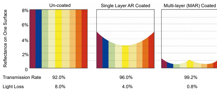
Transmission Comparison with White Clear Un-coated Lens
